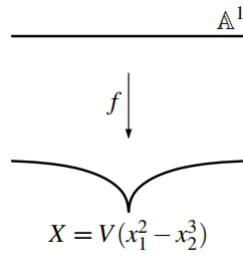
Figure 1.2: Isomorphisms \neq bijective morphisms.
