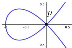
Figure 1.1: Plane cubic of equation x_2^2 - x_1^3 - x_1^2 = 0 , singular at the origin.
