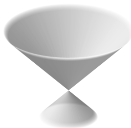
Figure 1.3: The light cone of N^1(X)
